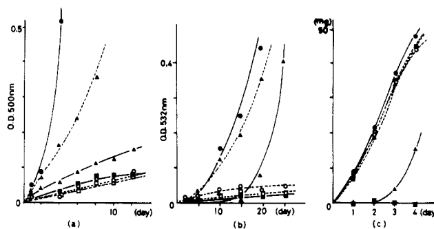
Figure 1. Antioxidative activity of the isolated antioxidants from E. globulus : (●) control; (▲) \alpha -tocopherol; (■) BHA; (□) n -tritriacontane-16,18-dione; (Δ) S-2A; (○) S-2B. (a) Thiocyanate method. (b) Thiobarbituric acid test (TBA method). (c) Weighing method.
