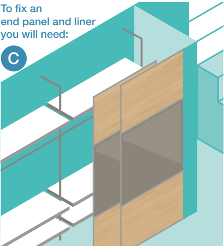
Wall to end panel
