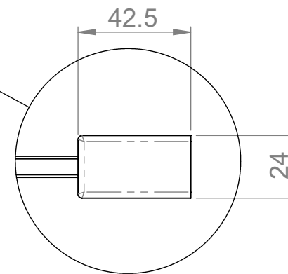
DETAIL D SCALE 1 : 2
